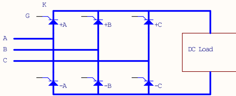
1. DC Converter
