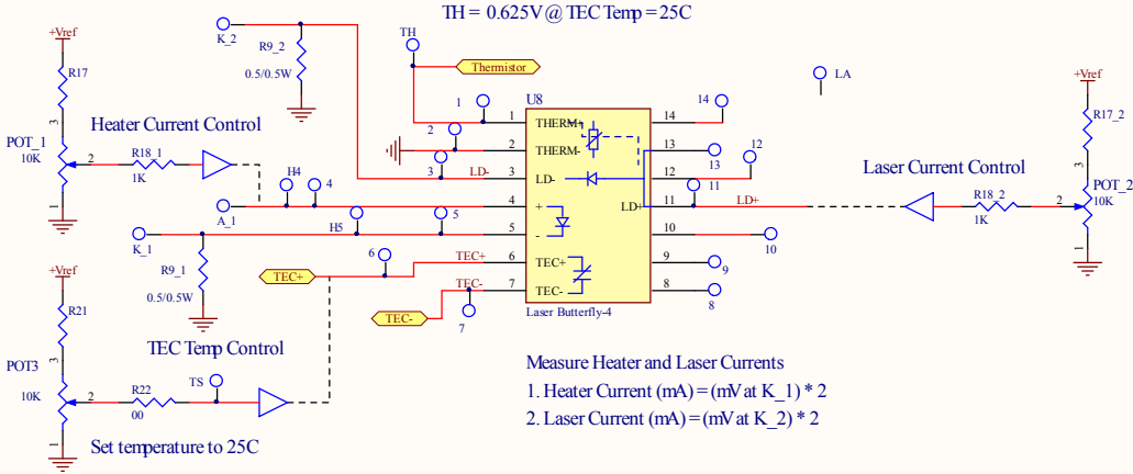
Laser, Heater & Temp Control Block Diagram
