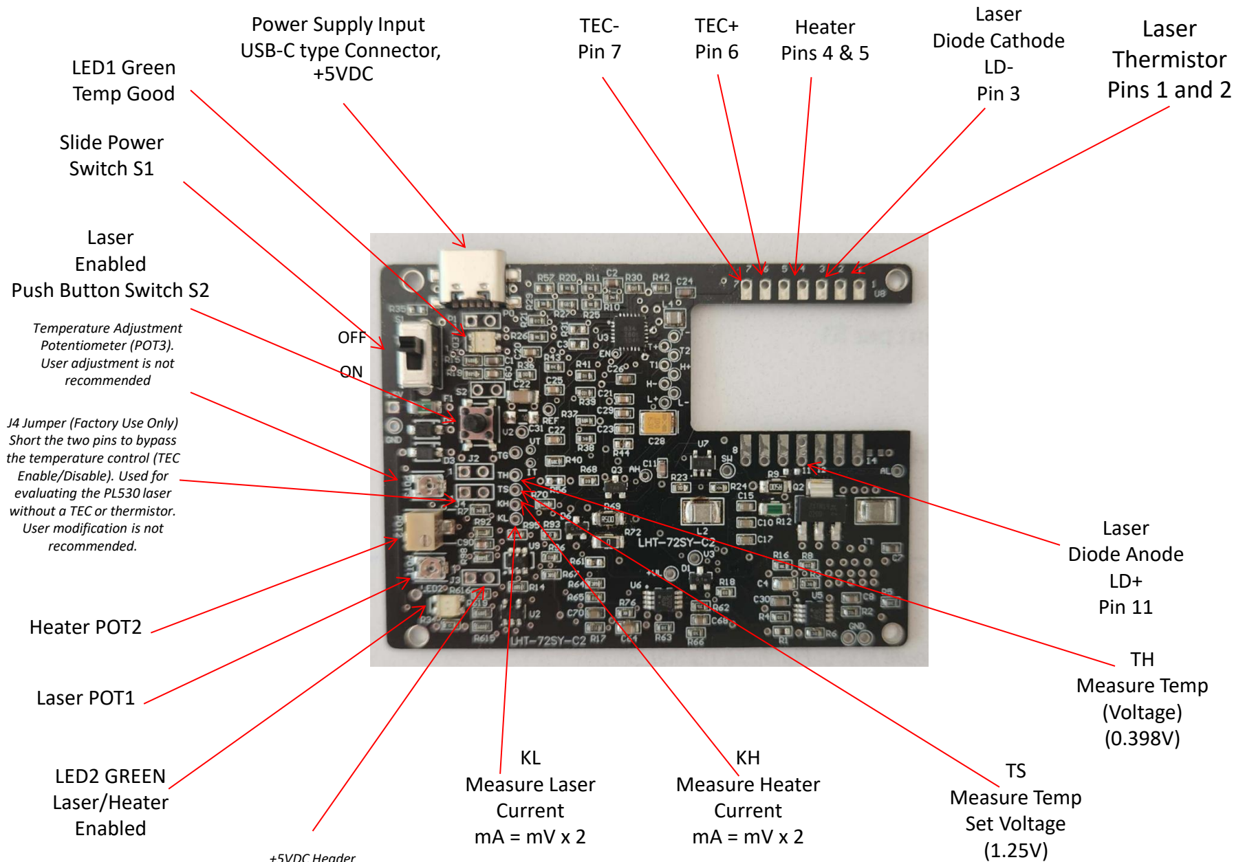
Pinout Rev C2
