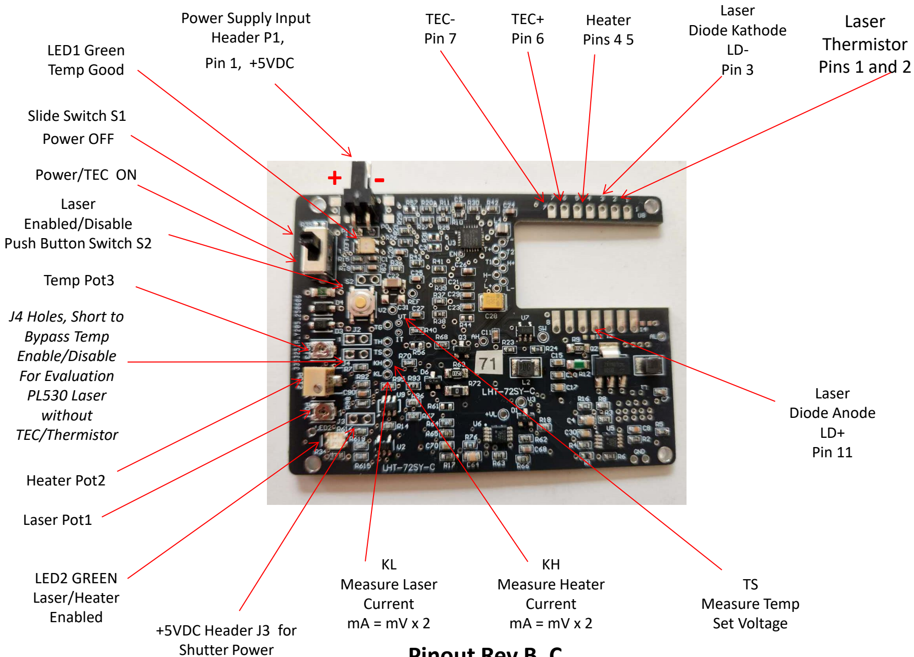
Pinout Rev B, C
